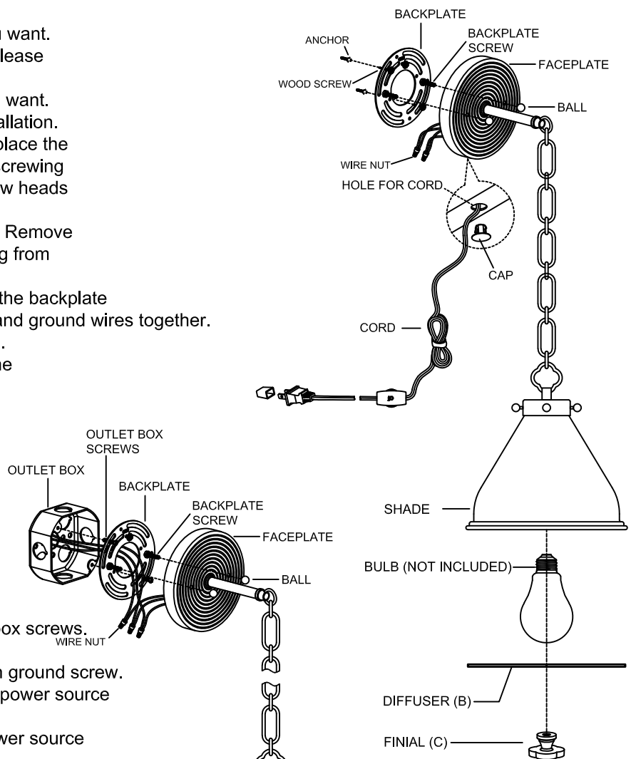
MOVABLE INSTALLTION METHOD
